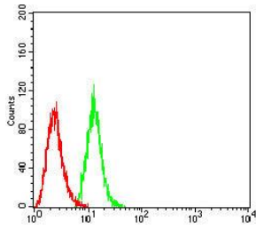
Flow cytometric analysis of THP-1 cells using CD7 mouse mAb (green) and negative control (red).
