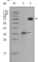
Western blot analysis using RET mouse mAb against truncated RET recombinant protein (1) and RET (aa658-1063)-hIgGFc transfected CHO-K1 cell lysate (2).
